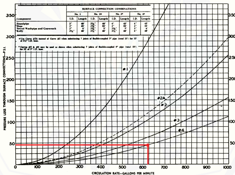
Gambar 3. Grafik Surface Connection Pressure Loss
