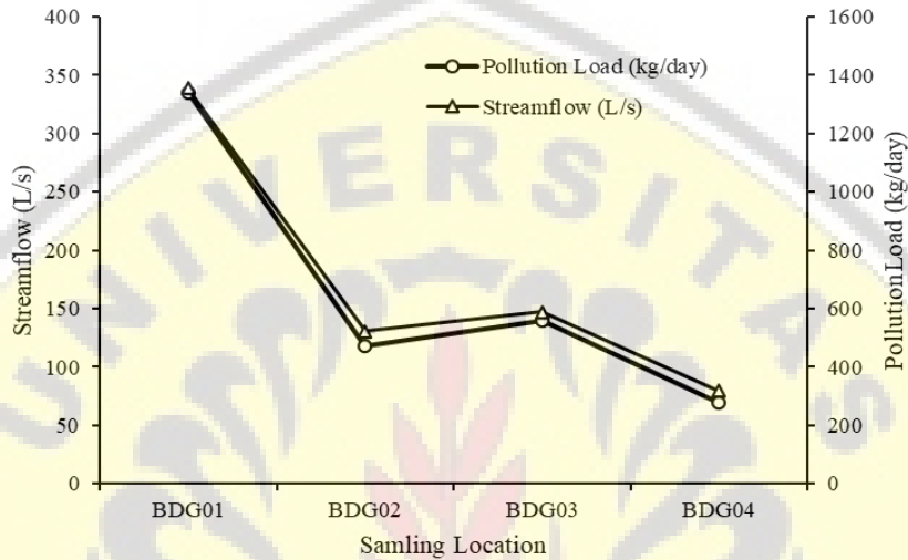
Figure 4 Streamflow graph at each sampling location of Bedagung River
