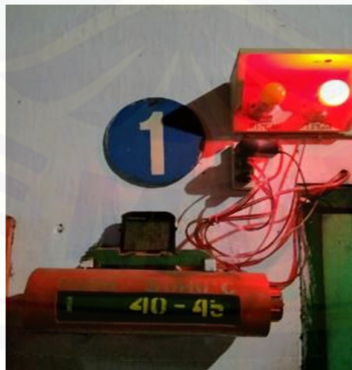
Fig 5. Lamp indicator when the smoking-room temperature is too high (red led is on)
