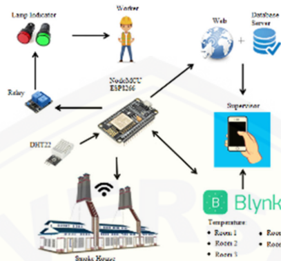
Fig 1. Working System of RSS Smoking Room Temperature Monitoring Device
