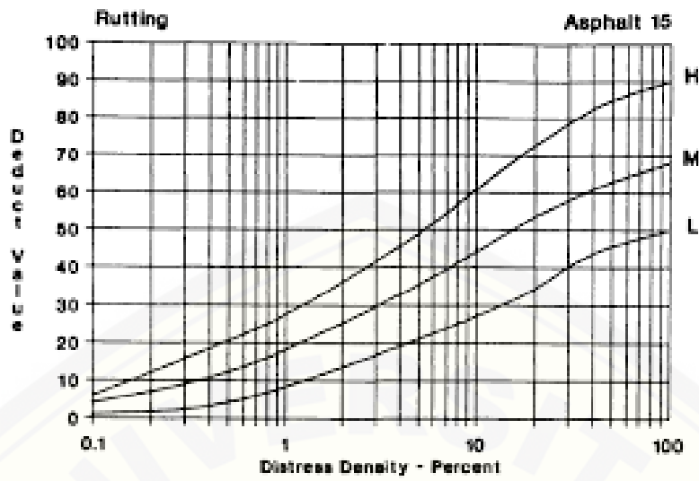
Gambar 2.27 Deduct Value Alur (Rutting) Sumber : Hardiyatmo, 2007
