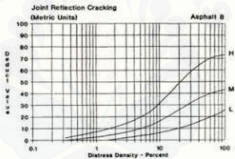
Gambar 2.22 Deduct Value Retak Sambungan ( Joint Reflection Cracking ) Sumber : Hardiyatmo, 2007
