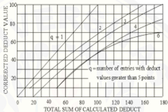
Gambar 2.29 Kurva Koreksi Nilai TDV dan Corrected Deduct Value , CDV Sumber: Shahin, 1994
