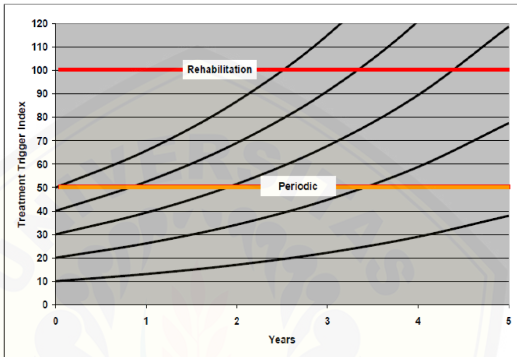
Gambar 2.17 Grafik Treatment Triggered Index (TTI)
