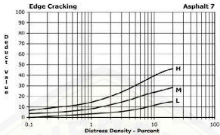
Gambar 2.21 Deduct Value Cacat Tepi Perkerasan ( Edge Cracking ) Sumber : Hardiyatmo, 2007
