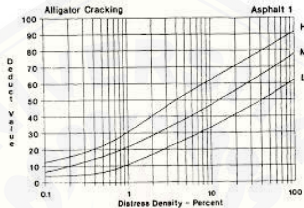
Gambar 2.19 Deduct Value Retak Kulit Buaya ( Alligator Cracks ) Sumber : Hardiyatmo, 2007
