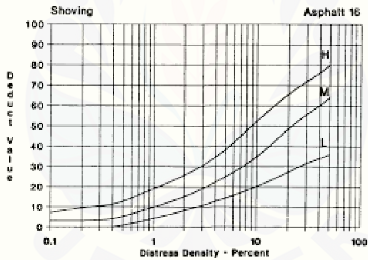
Gambar 2.28 Deduct Value Sungkar (Shoving) Sumber : Hardiyatmo, 2007
