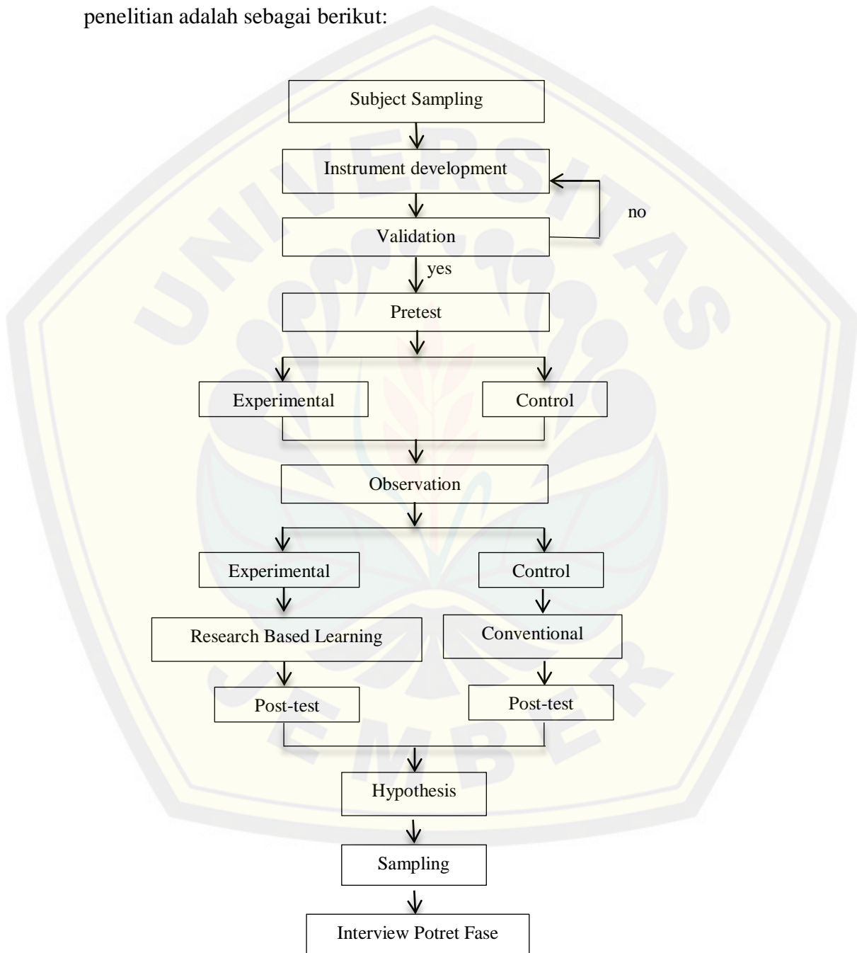
Gambar 3.2 Prosedur Penelitian
