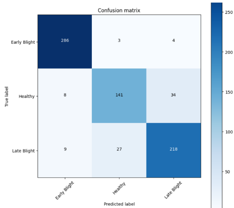
Gambar 4.9 Confusion Matrix Arsitektur Inception ResnetV2
