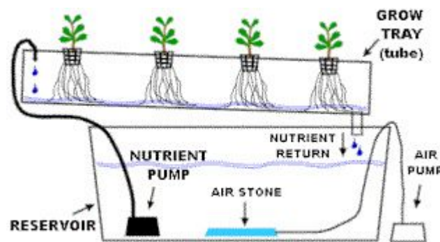
Gambar 2.3 Sistem Hidroponik Nutrient Film Technique (Sumber: http://media-cache-ak0.pinning.com )
