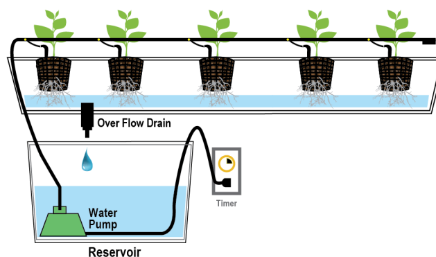
Gambar 2.4 Sistem Hidroponik Drip-Irrigation (Sumber: http://media-cache-ak0.pinimg.com )
