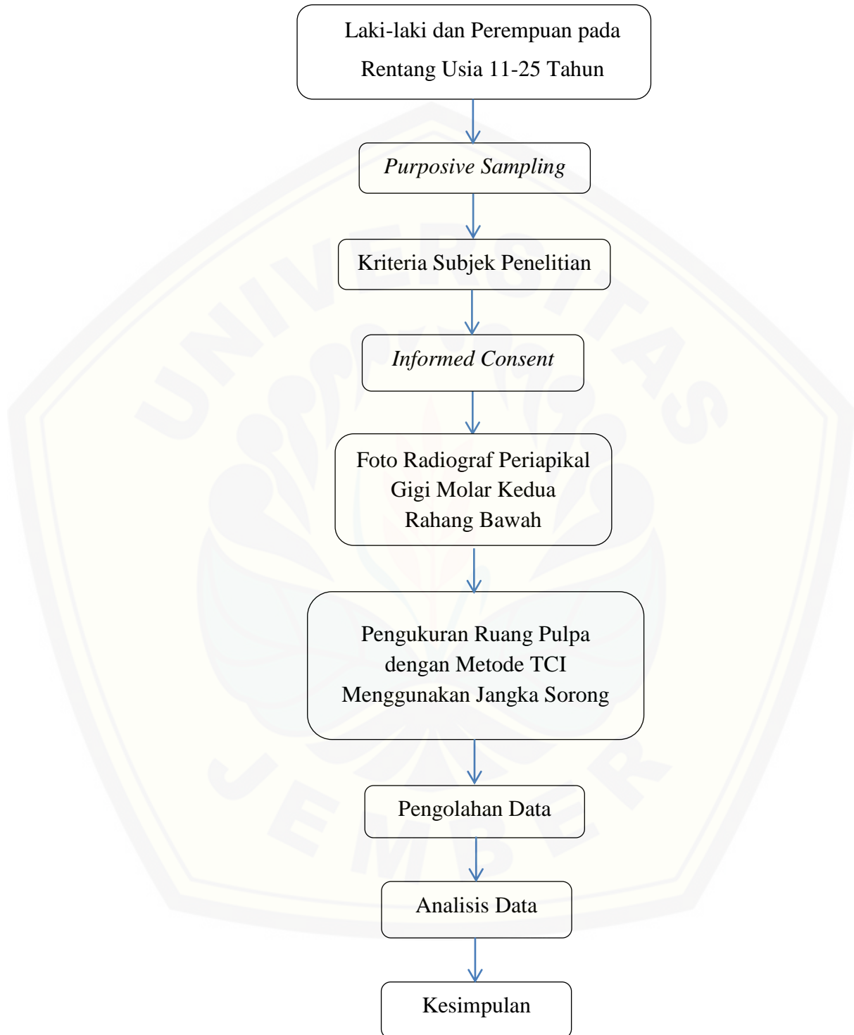
Gambar 3.2 Alur Penelitian
