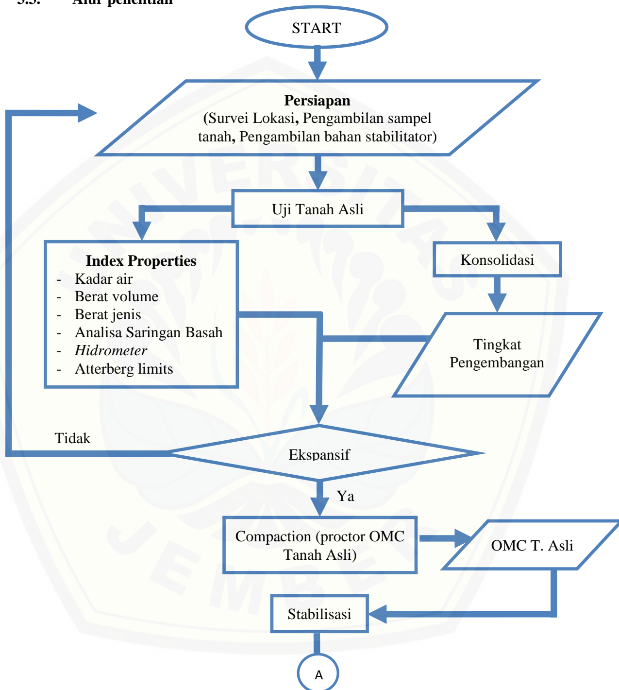
Gambar 3. 2 Alur Penelitian
