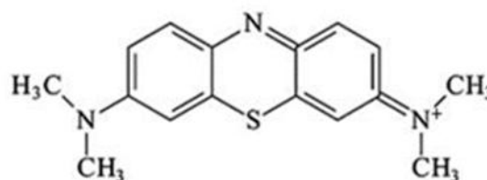
Figure 1. Chemical structure of Methylene Blue
