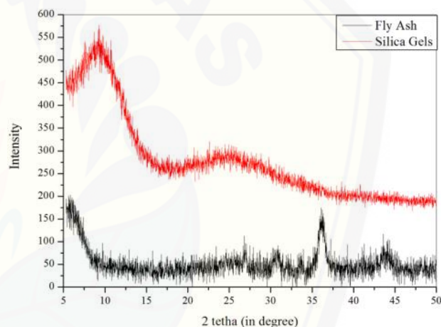
Figure 3. The X-Ray diffractogram of materials
