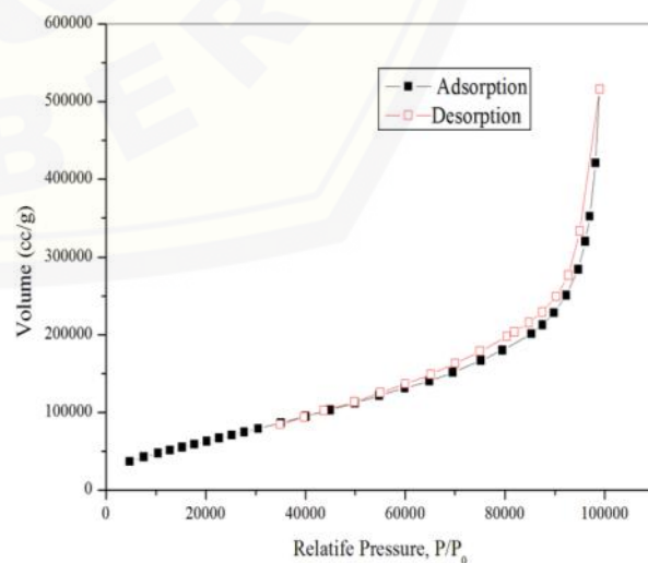
Figure 5. Isothermal adsorption-desorption N 2 of silica gels
