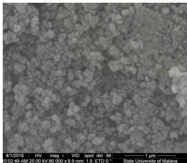
Figure 4. The surface morphology of silica gels
