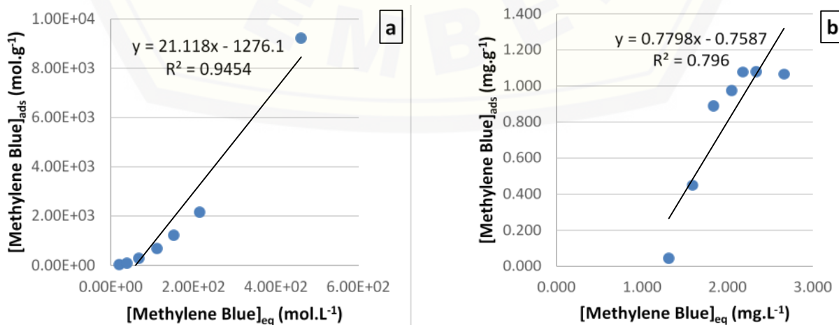
Figure 8. Isothermal adsorption methylene blue on fly ash using models: a) Langmuir; b) Freundlich
