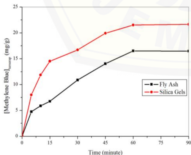
Figure 9. The isothermal adsorption of methylene blue on various time interaction
