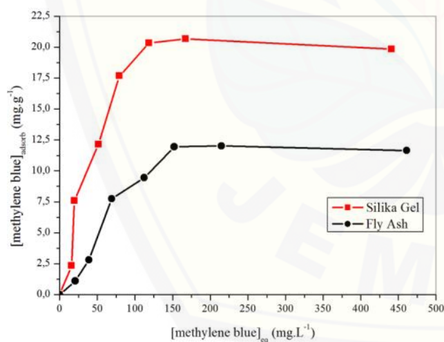
Figure 6. The adsorption isotherm materials on various methylene blue concentration
