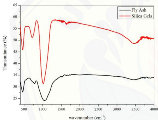
Figure 2. FT-IR spectra of materials
