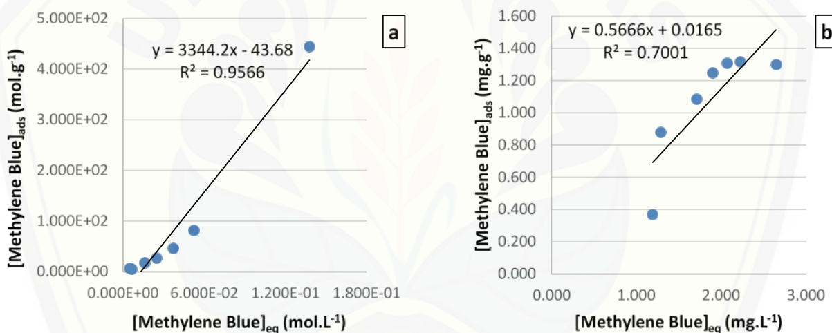
Figure 7. Isothermal adsorption methylene blue on silica gels using models: a) Langmuir; b) Freundlich
