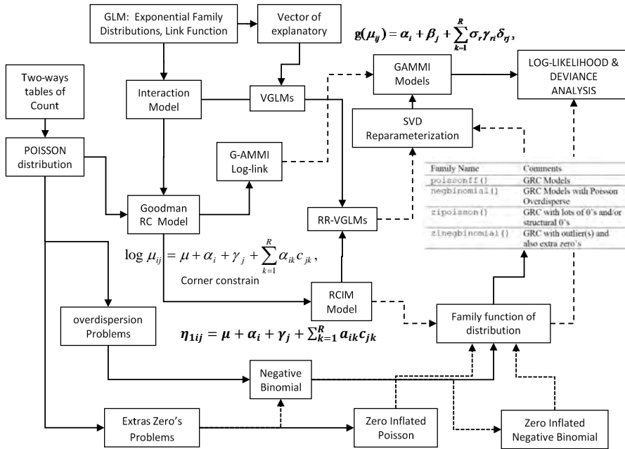
Figure 1: Statistical framework of The RCIM
