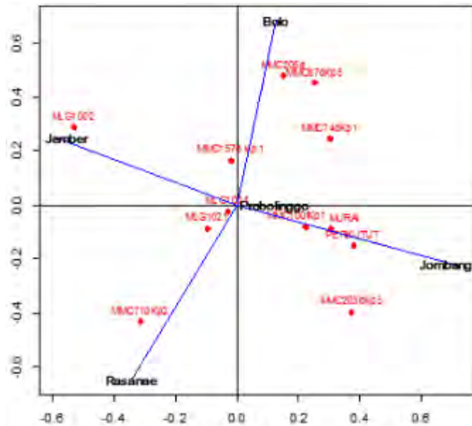
Figure 4: Biplot of the interaction effect on Log-scale of Zero-inflated Poisson
