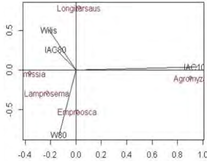
Figure 2: The Biplot of RCIM rank=2 for endurance of varieties of soybean to some leaf pests.
