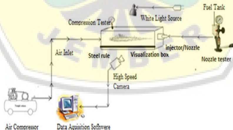
Figure 1. Experiment setup scheme
