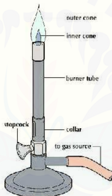
Gambar 3.6 Bunsen Burner
